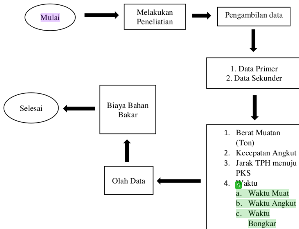
Gambar 1. Flowchart
